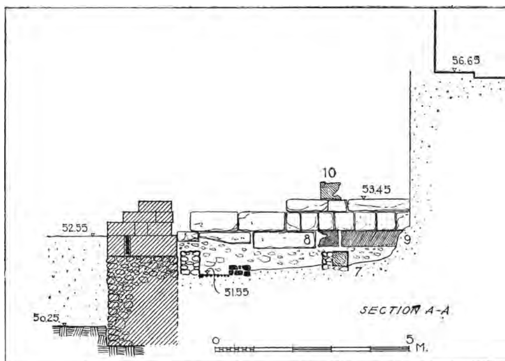
Fig. 3. Section A-A of the Plan Fig. 2.
